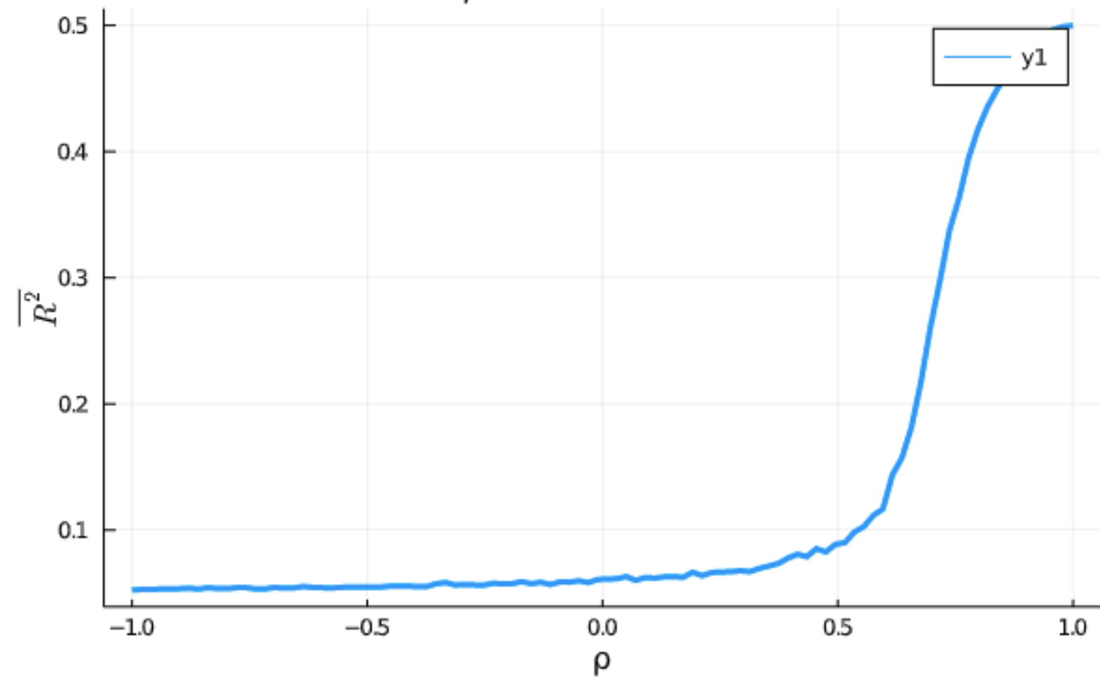
\overline{R^2} vs. \rho for 20-Oscillator Grid
